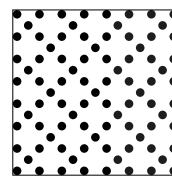
Acoustiroc® ASTRAL 17% Ø2.5 (round, regular) \alpha_w = 0.95 NRC : 0.90
